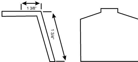
.045 x 2 1 / 4 " x 3 1 / 8 " Series 90 Standard Sold-Out Paddle Short 432,070,29x.x3
